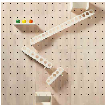
STEM Ball Drop 4 flush mount pins 8 non-locking pins (.5" PVC)
